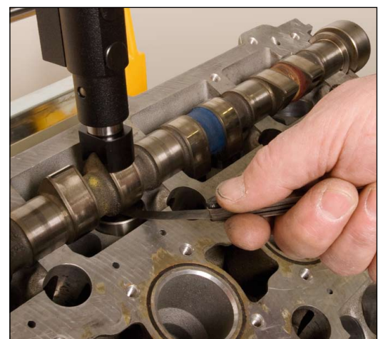
Valve clearance pressure foot and stop collar. For valve clearance adjustment without to install cam shaft bearing caps.
